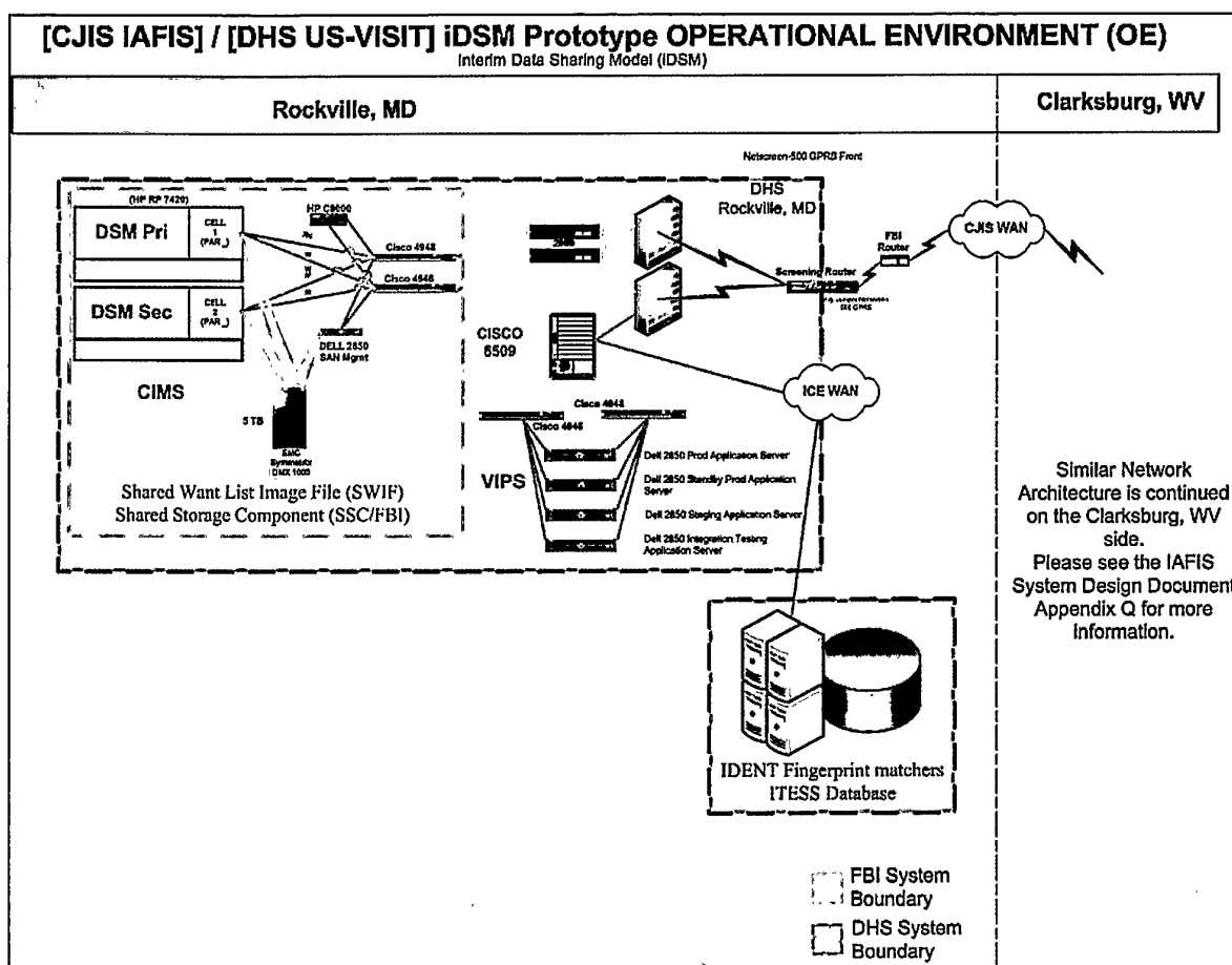
Figure 4.1.1-1 Example of a iDSM Network Enclave
