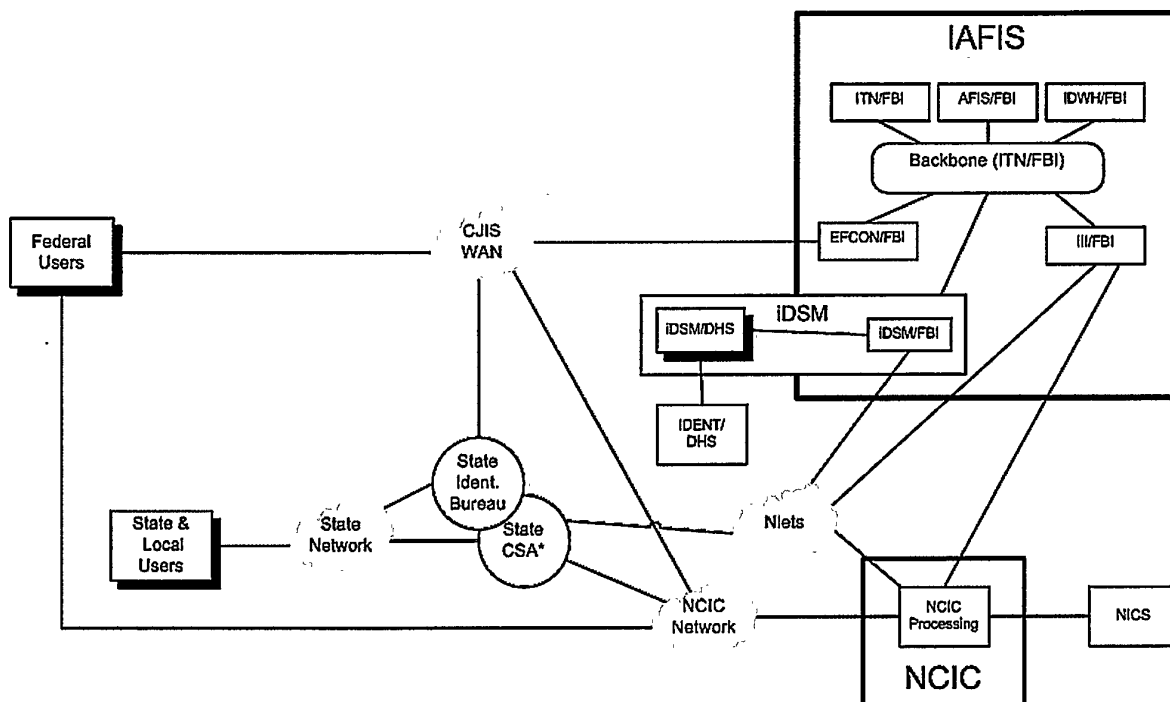
Figure 3.1-1 IAFIS Full Operational Capability Architecture
