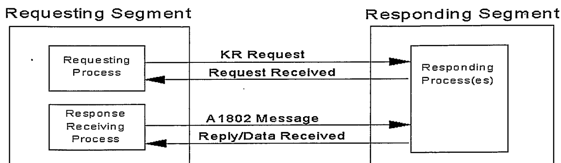
Figure 4.9.5.1-4 Use of A1802 With KR Protocol – Normal Response
