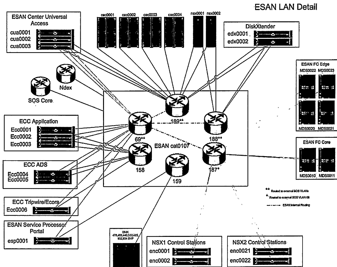
Figure J.5.1 Hardware Diagram
