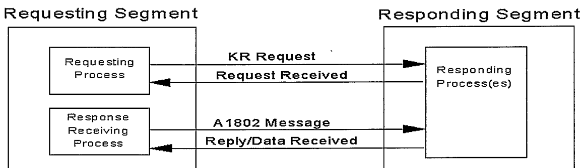
Figure 4.9.5.1-3 Use of A1802 With KR Protocol – Response Error
