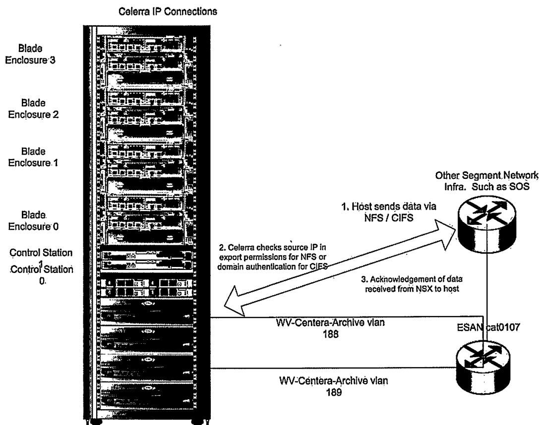
Figure J.6.7.1 Multi-Protocol File Sharing
