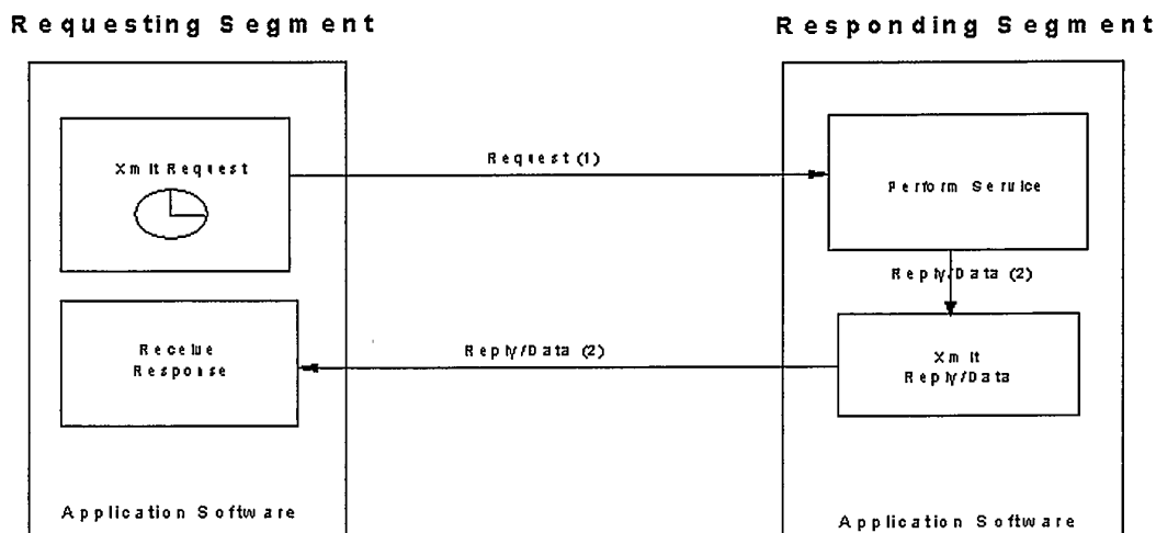
Figure 3.2.3-1 Immediate Request Protocol With Response Time-Out Clock Added
