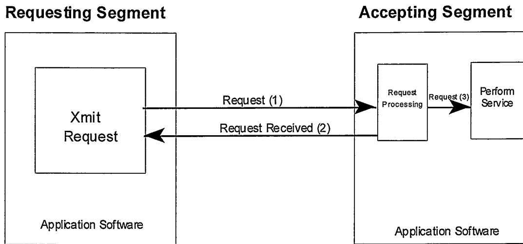
Figure 3.2.1.3-1 Basic No Response Intersegment Service Request Protocol
