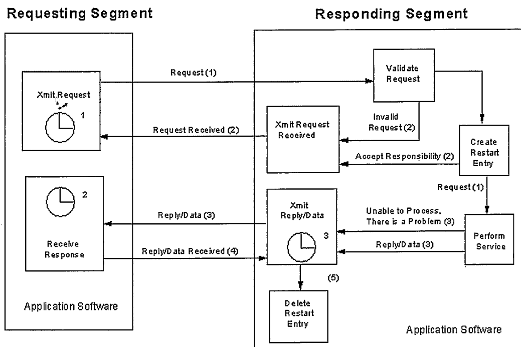
Figure 3.2.6-2 Complete Queued Response Protocol Including Exception and Error Handling
